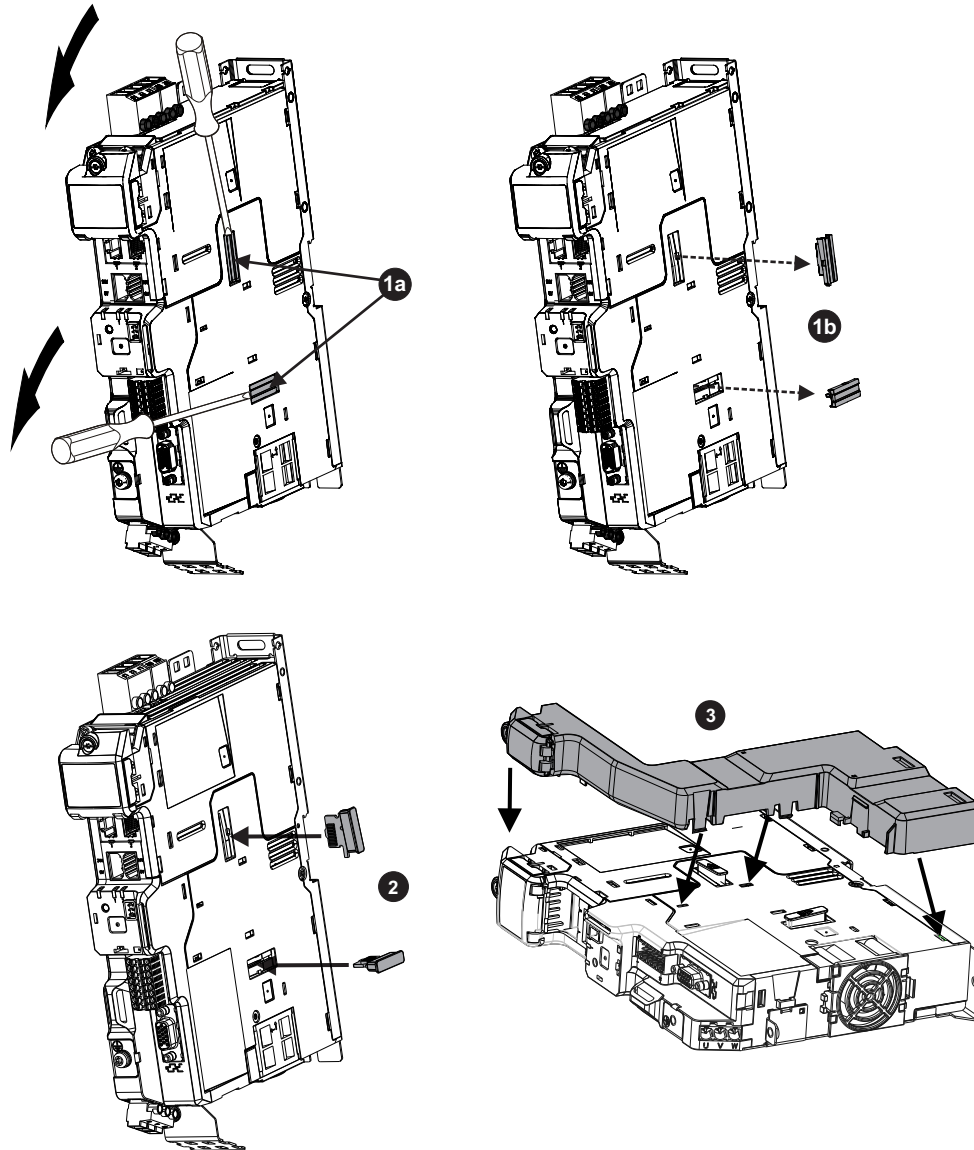
Figure 1-1 SI-Option Mounting kit installation
