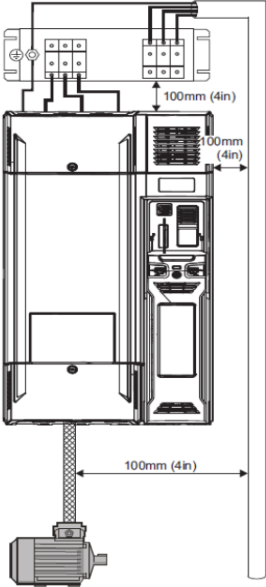
Figure.4 Wire spacing
