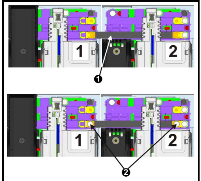
Figure 1-5 Installing the DC - busbar
