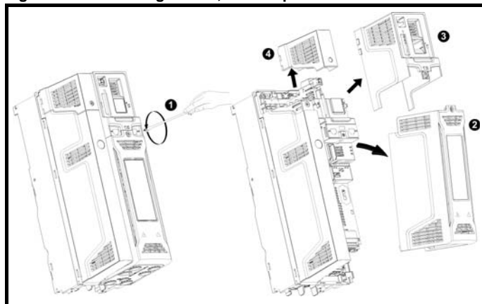
Figure 1-1 Removing the AC, DC and power terminal covers
