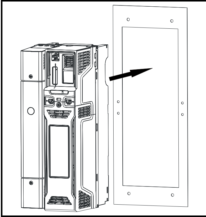
Figure 3-4 Position the drive through the backplate
